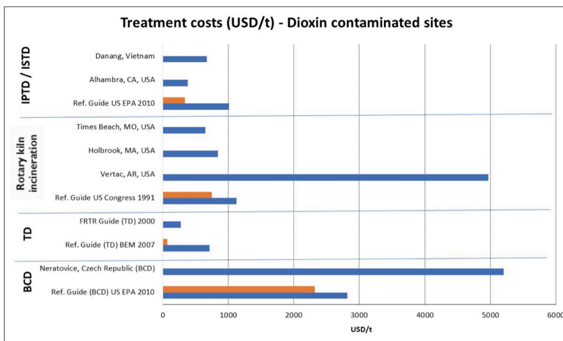
Figure 9: Treatment costs (USD/t) – Dioxin Contaminated Sites
